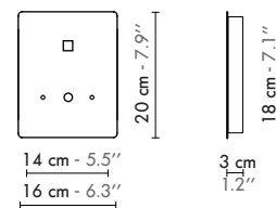
Wall plate
