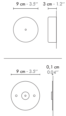
Wall plate
