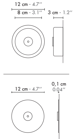
Wall plate
