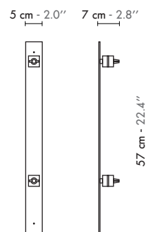
Wall plate
