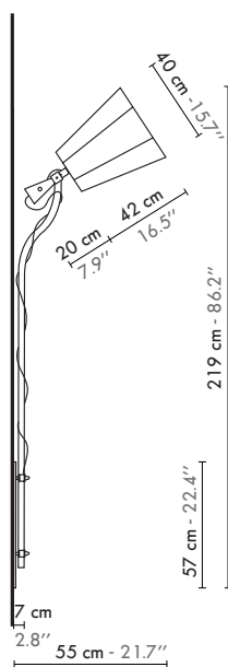
Body
