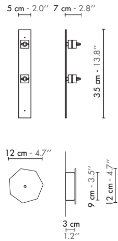
Wall plate
