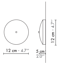
Wall plate
