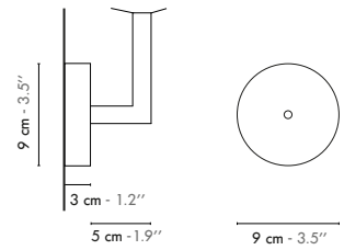
Wall plate
